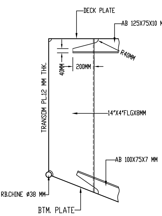
3-DETAIL
