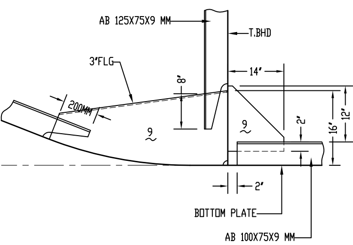
4-DETAIL
