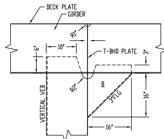
2-DETAIL
