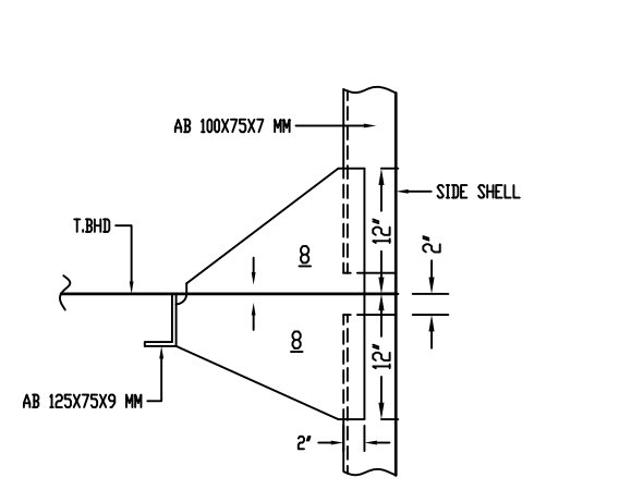
B-B SECTION
