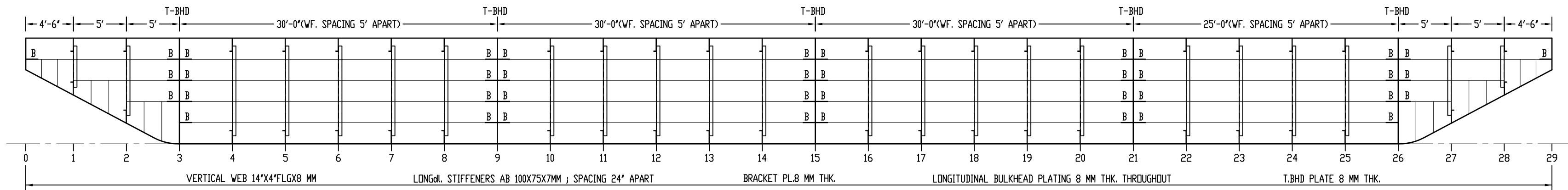
SECTION AT LONGd. BULKHEAD (CENTER LINE)
