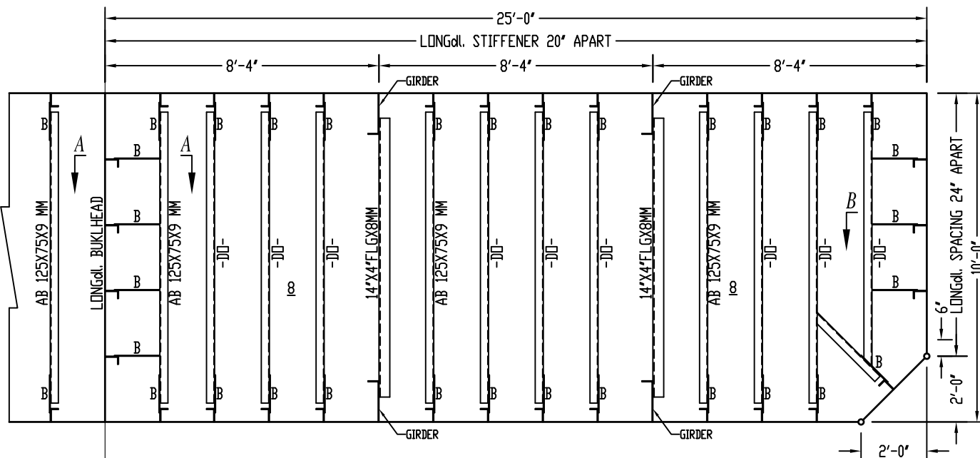
TRANSVERSAL BULKHEAD SECTION(TYP)
