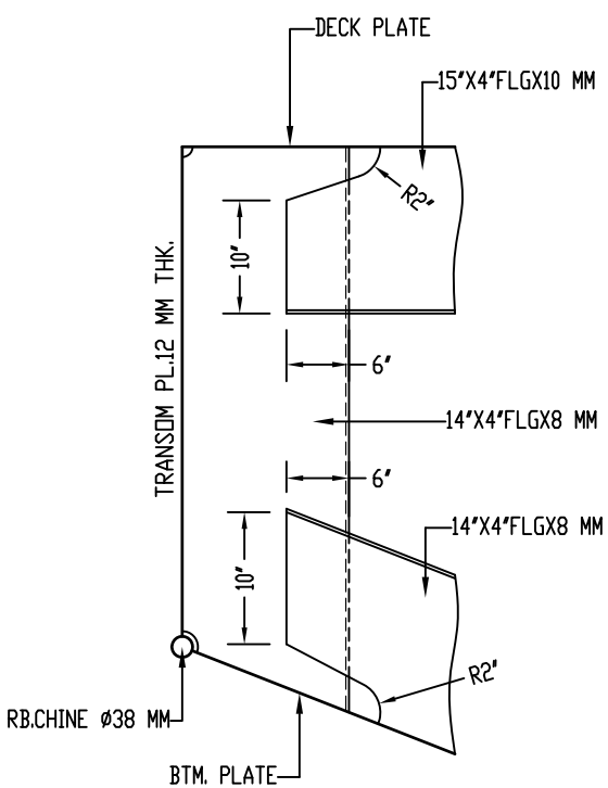
1-DETAIL
