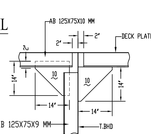
5-DETAIL
