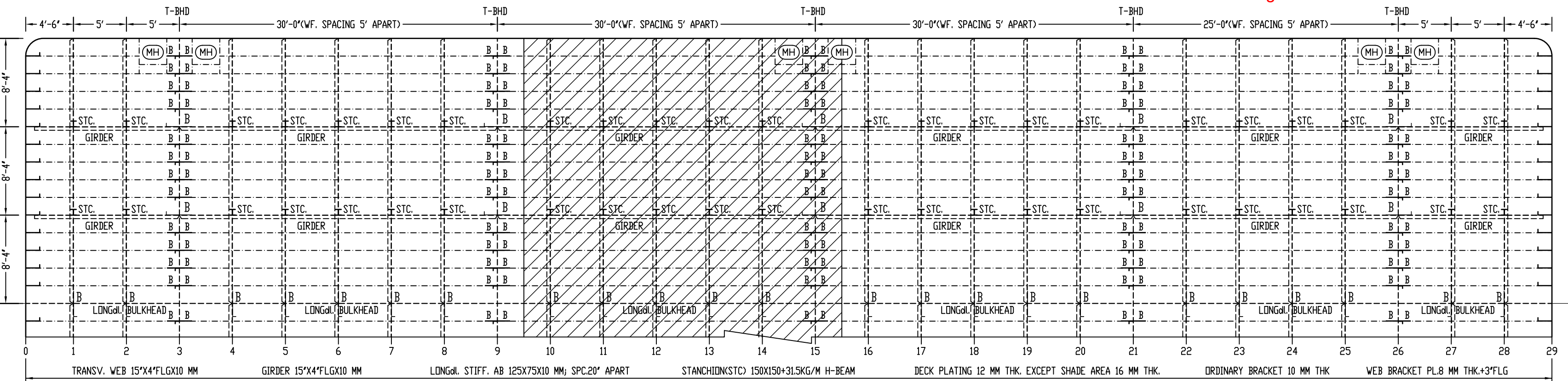
DECK PLAN
