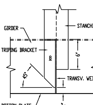
C-C SECTION
