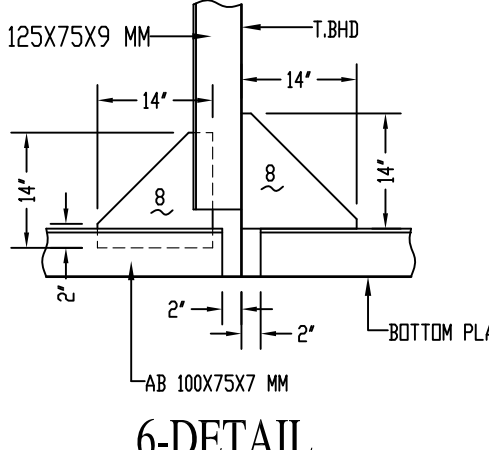
6-DETAIL
